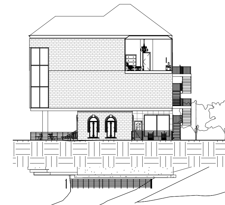
4 North -- COVER SHEET 3/64" = 1'-0"
