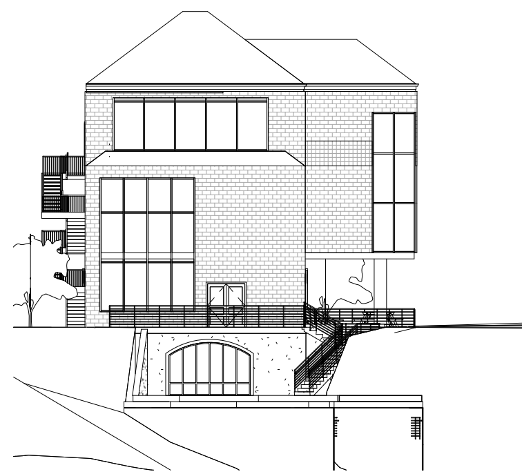
5 South COVER SHEET 3/64" = 1'-0"
