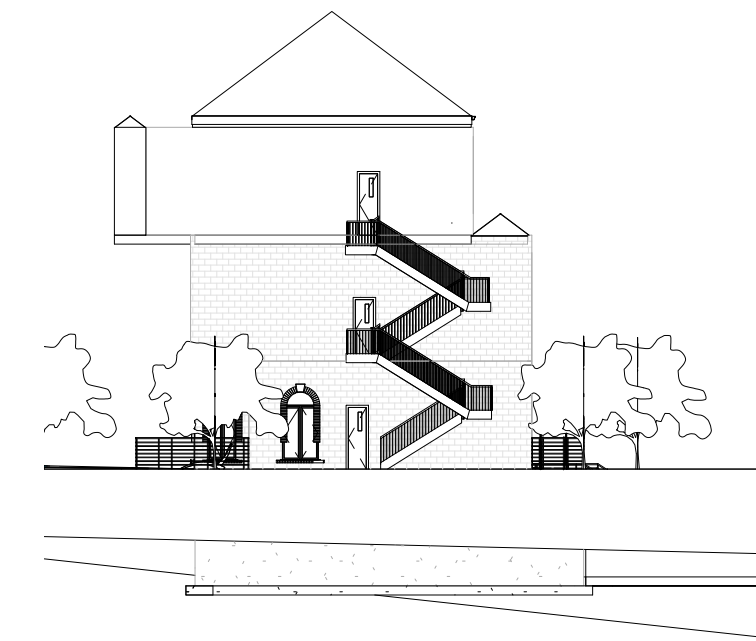
③ West -- COVER SHEET 3/64" = 1'-0"
